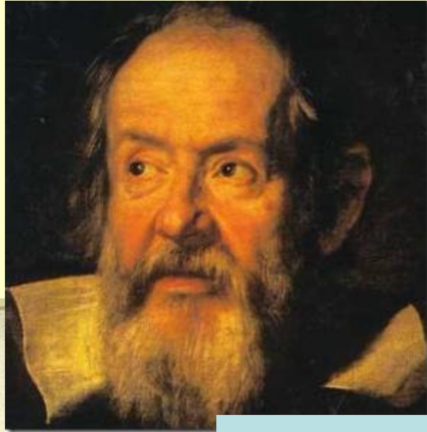
Galileo Galilei (1564-1642)
